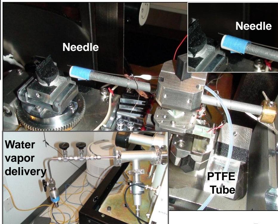
Prototype Nanomanipulator and gas delivery system built by Xidex
