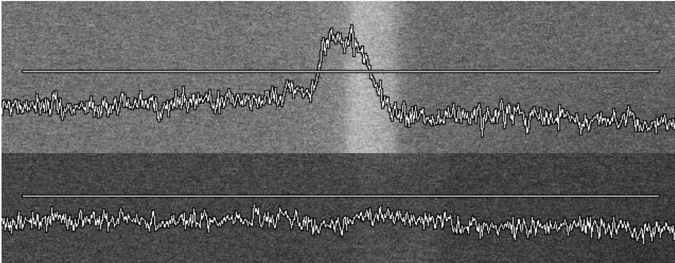
Secondary electron imaging example during line scanning across a CNT (top) and after CNT is cut (bottom)
