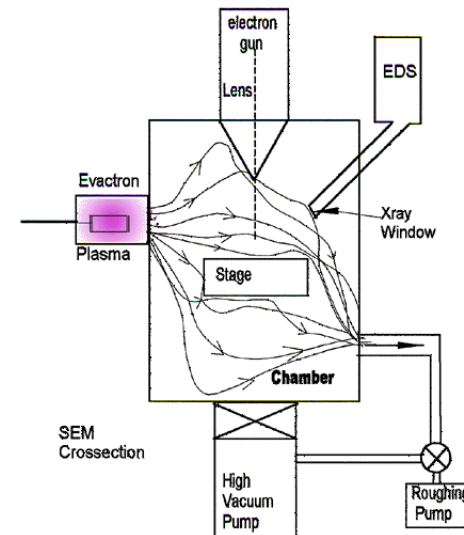
XEI Scientific EVACTRON™ system schematic
